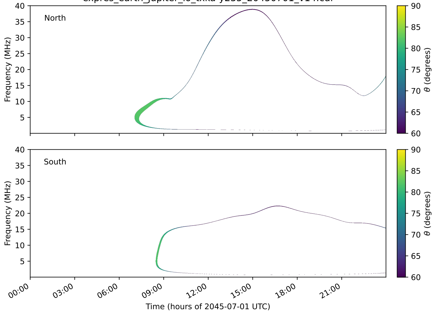
expres_earth_jupiter_io_txka-y235_20450701_v14.cdf
