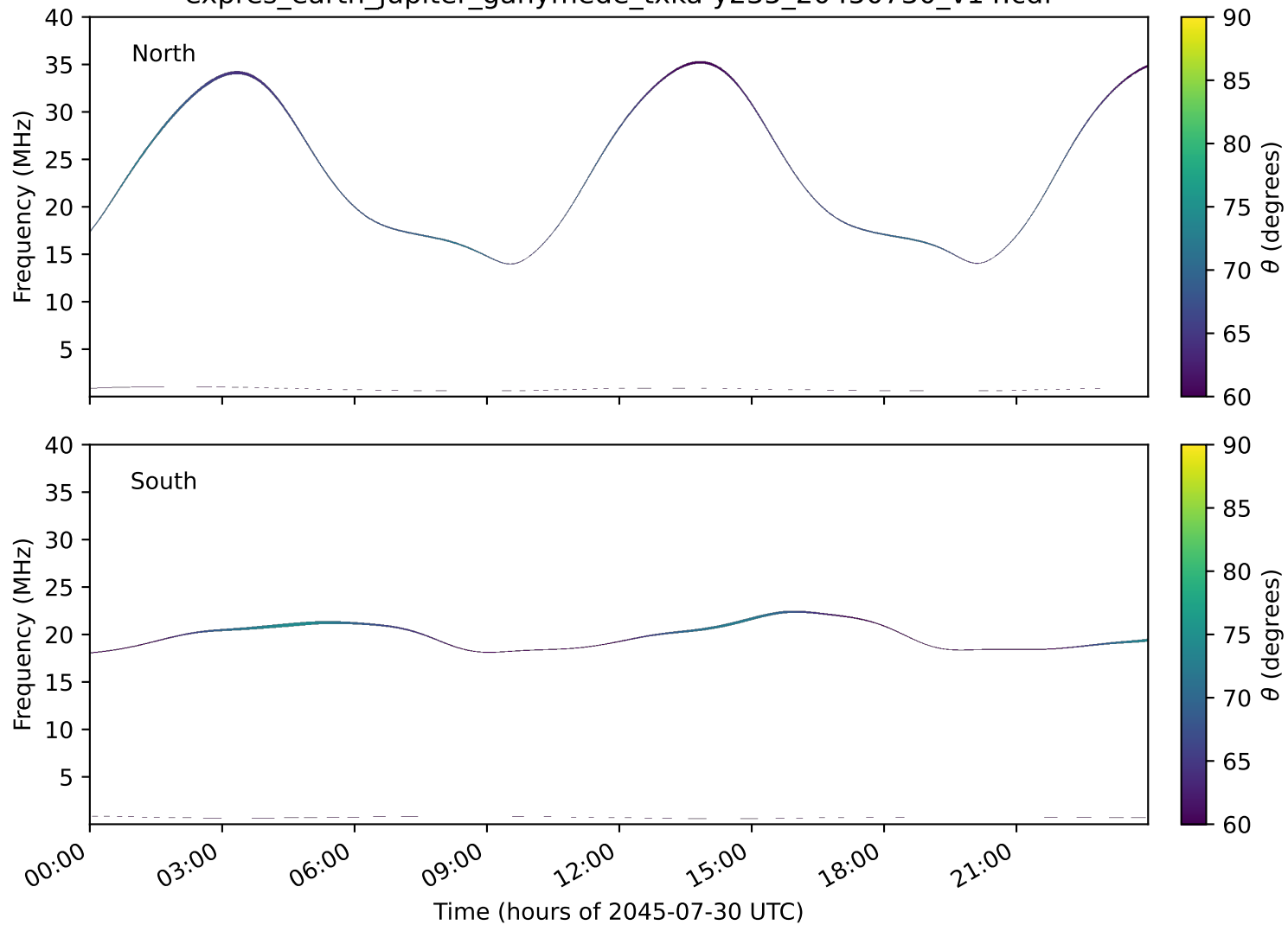
expres_earth_jupiter_ganymede_txka-y235_20450730_v14.cdf
