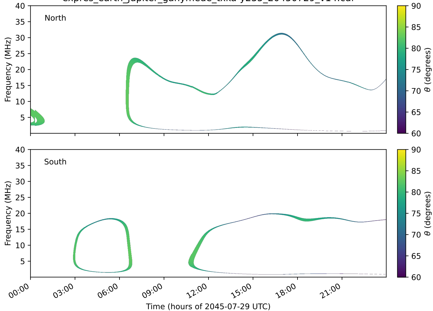
expres_earth_jupiter_ganymede_txka-y235_20450729_v14.cdf
