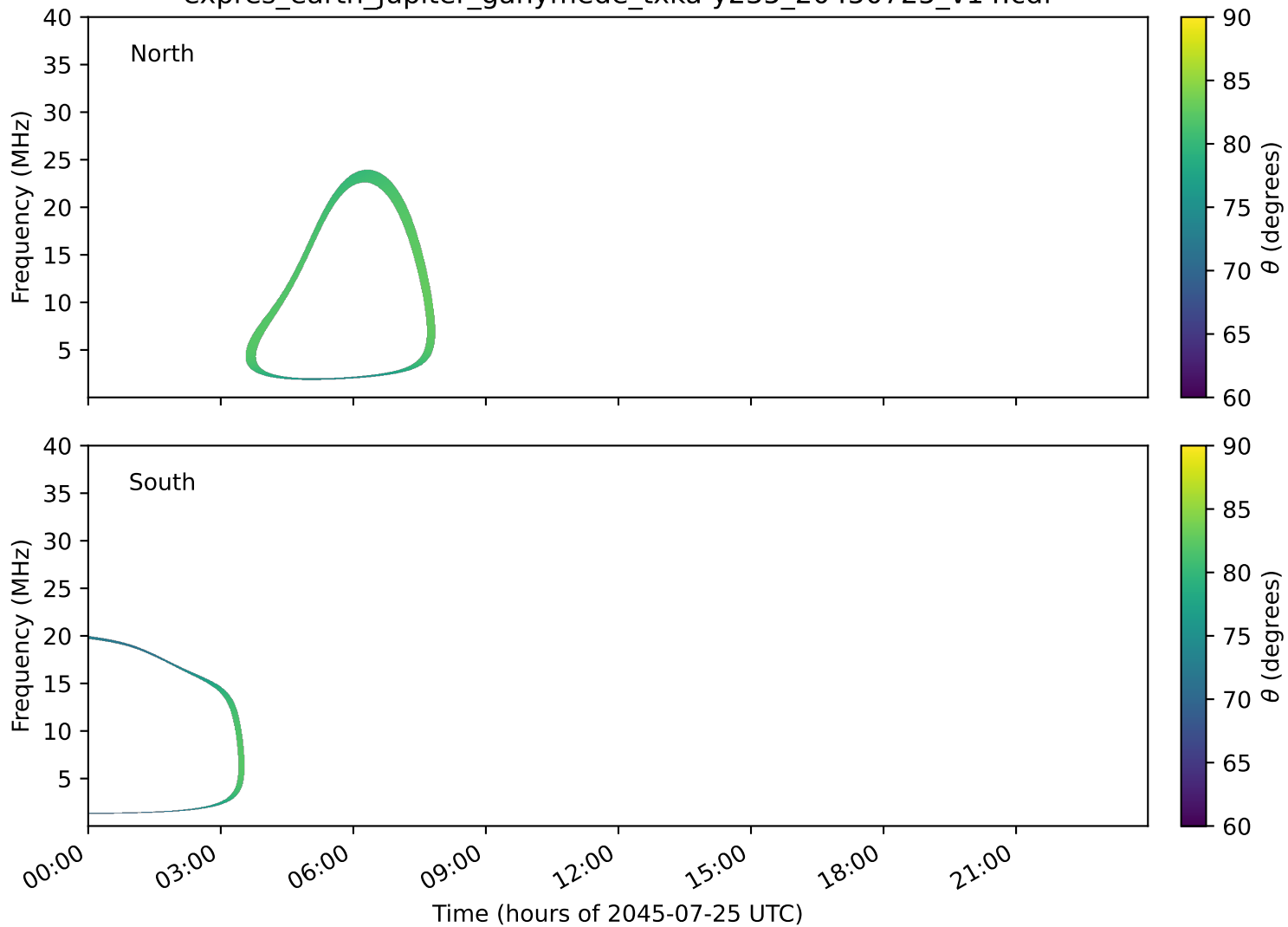
expres_earth_jupiter_ganymede_txka-y235_20450725_v14.cdf
