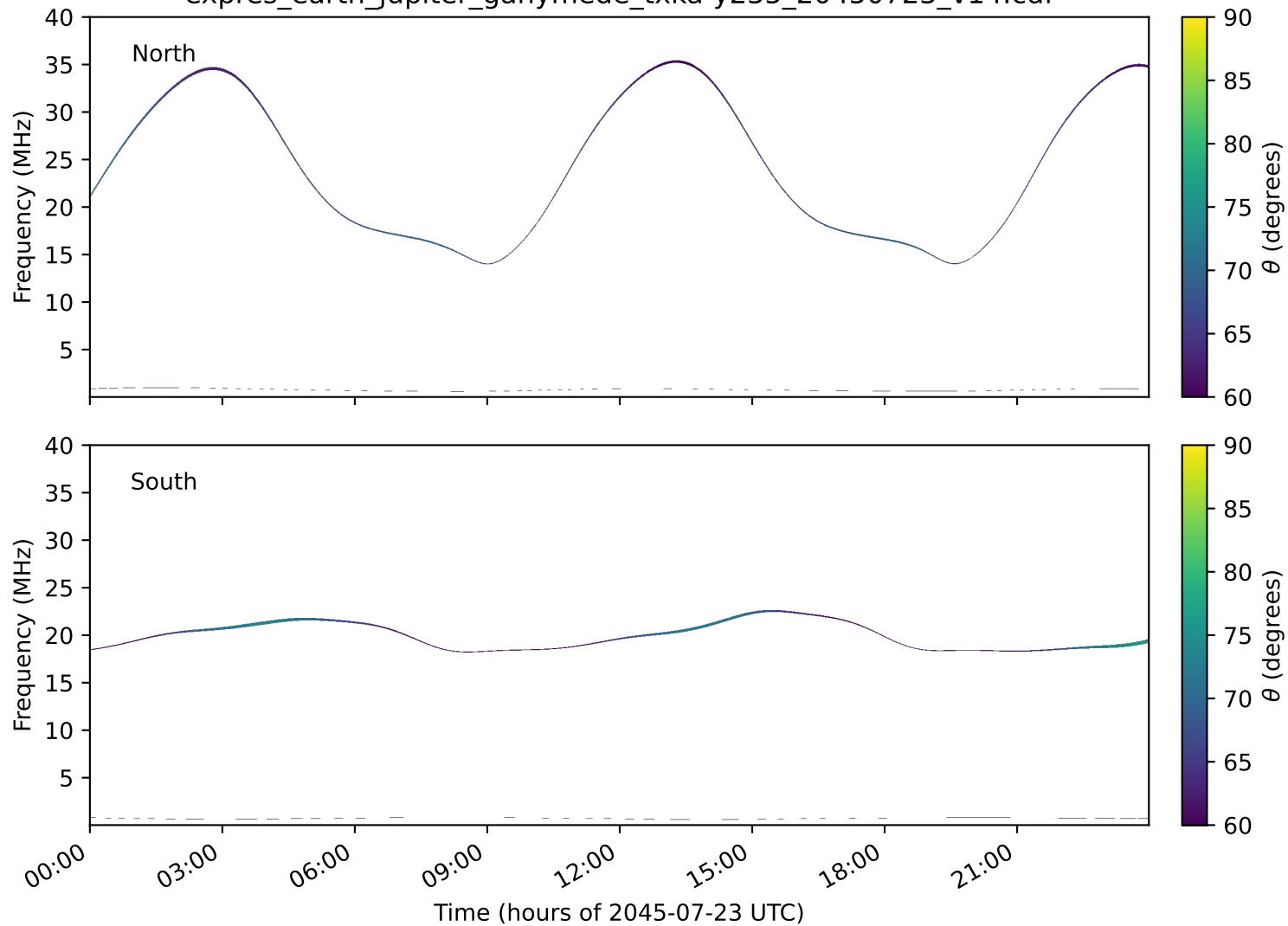
expres_earth_jupiter_ganymede_txka-y235_20450723_v14.cdf
