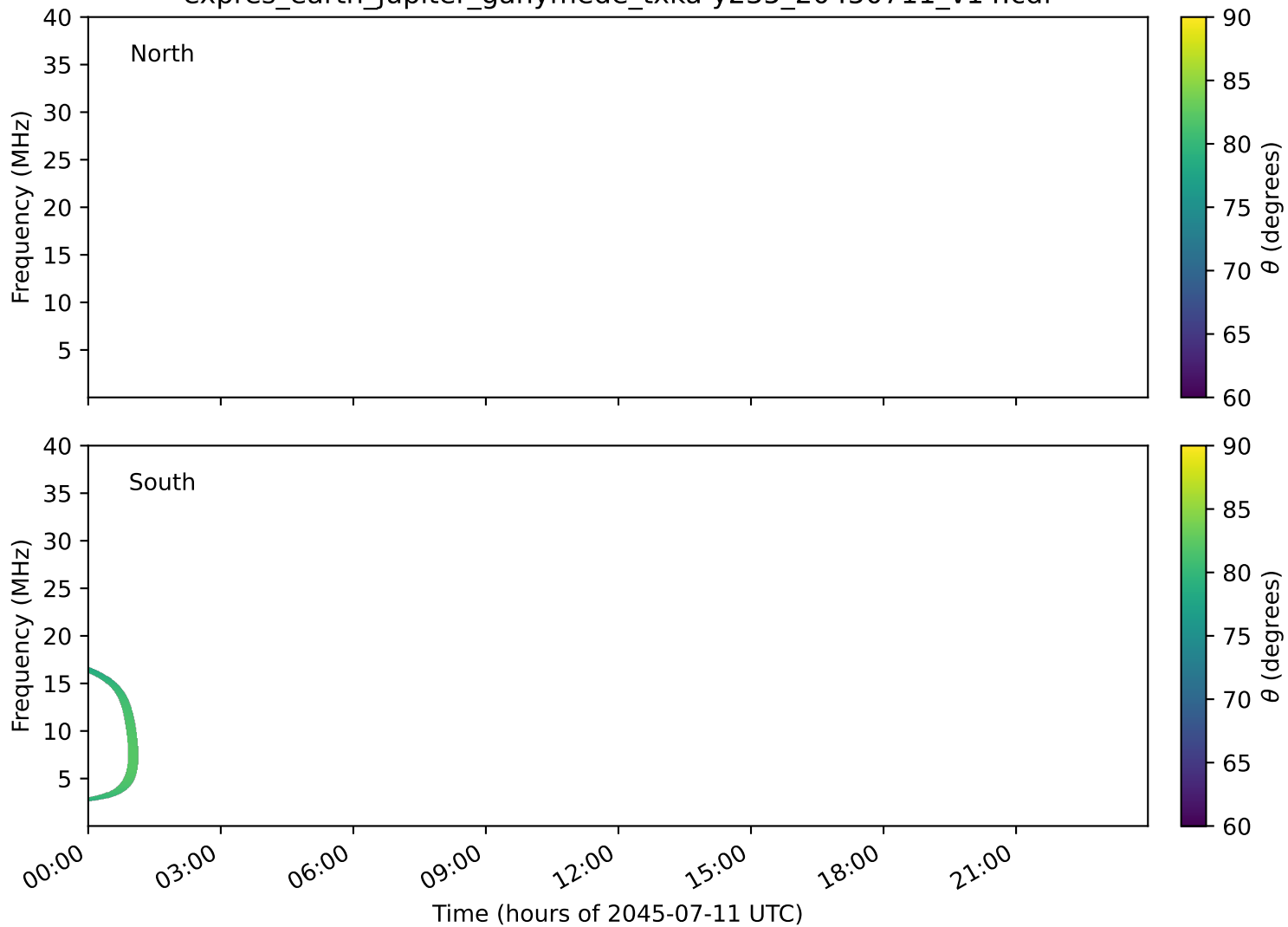
expres_earth_jupiter_ganymede_txka-y235_20450711_v14.cdf
