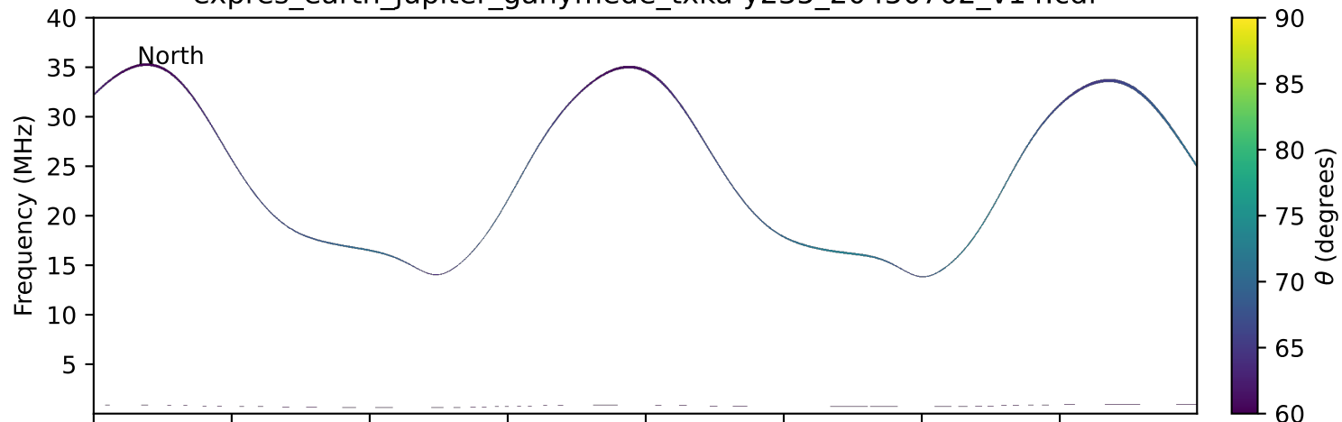
expres_earth_jupiter_ganymede_txka-y235_20450702_v14.cdf
