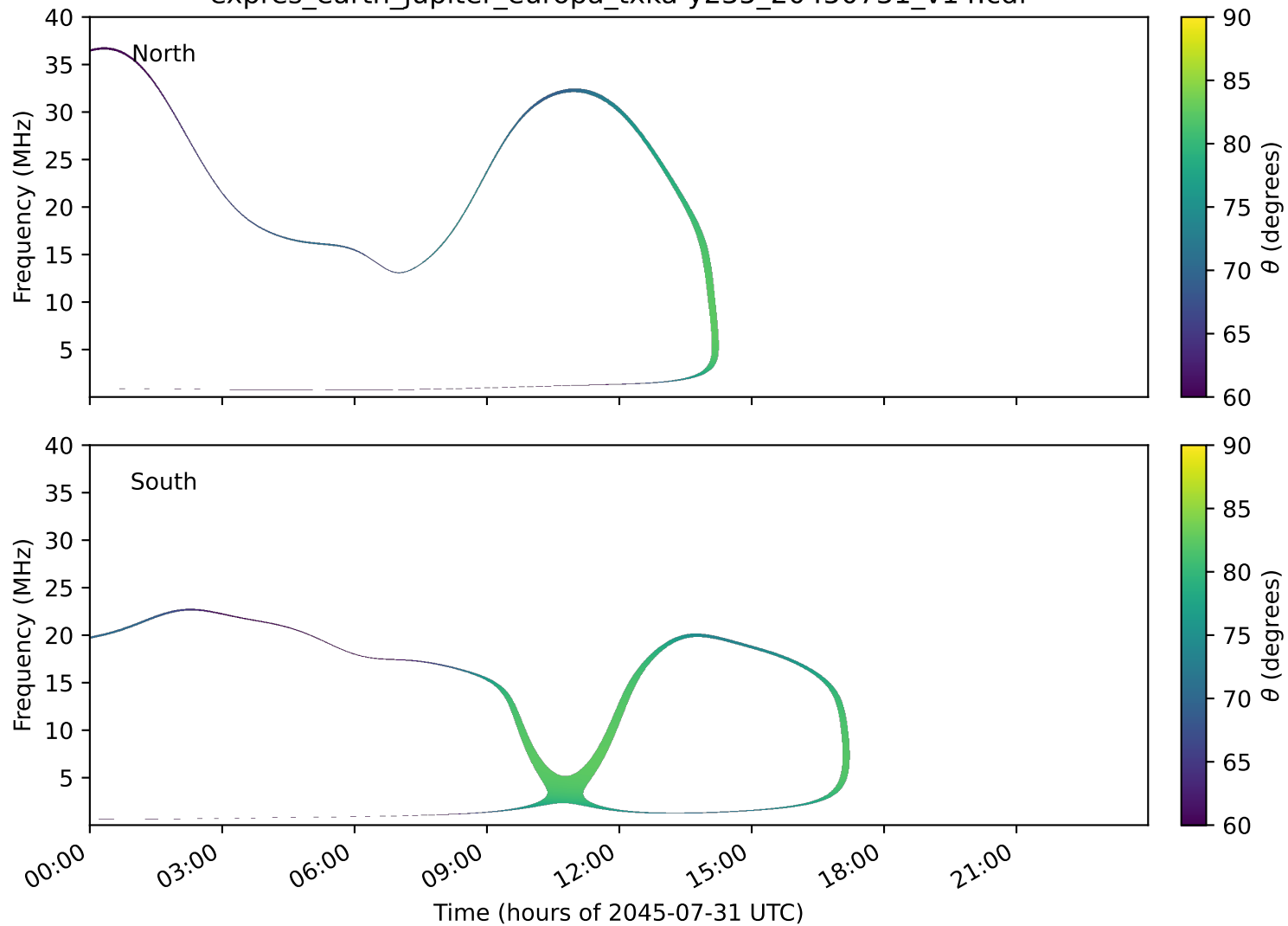
expres_earth_jupiter_europa_txka-y235_20450731_v14.cdf
