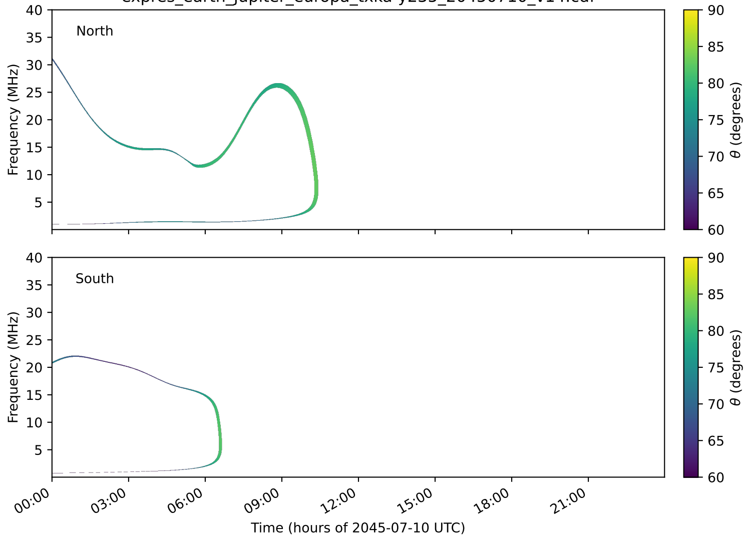
expres_earth_jupiter_europa_txka-y235_20450710_v14.cdf
