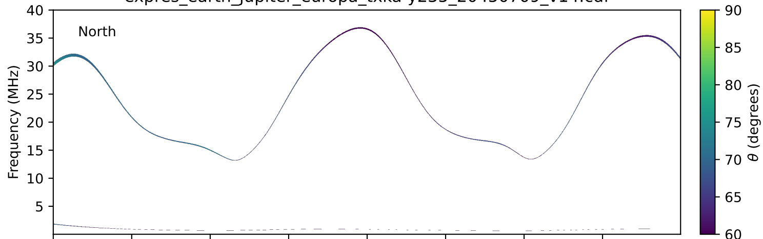
expres_earth_jupiter_europa_txka-y235_20450709_v14.cdf
