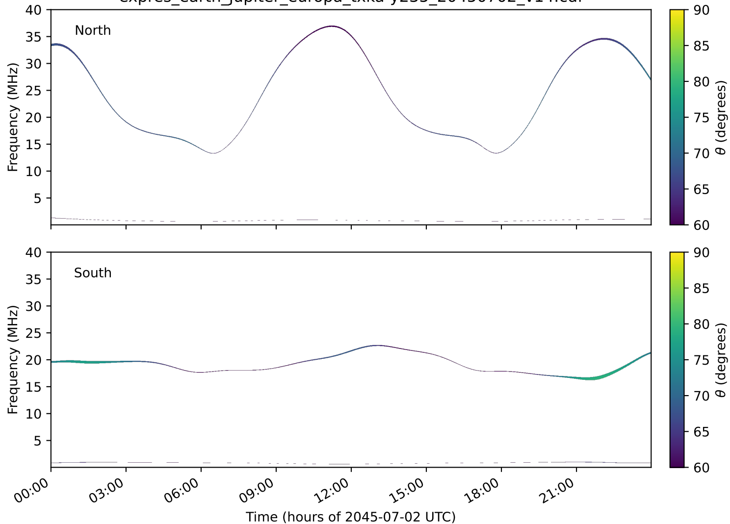
expres_earth_jupiter_europa_txka-y235_20450702_v14.cdf
