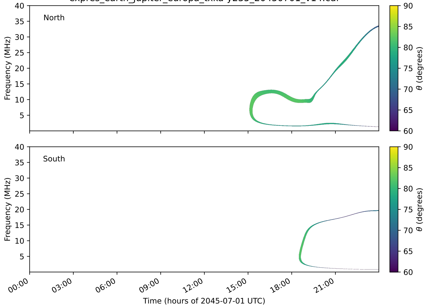
expres_earth_jupiter_europa_txka-y235_20450701_v14.cdf
