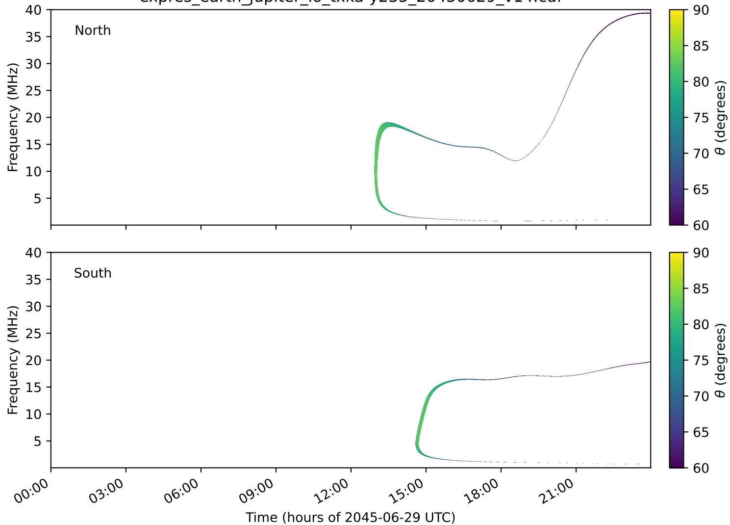
expres_earth_jupiter_io_txka-y235_20450629_v14.cdf
