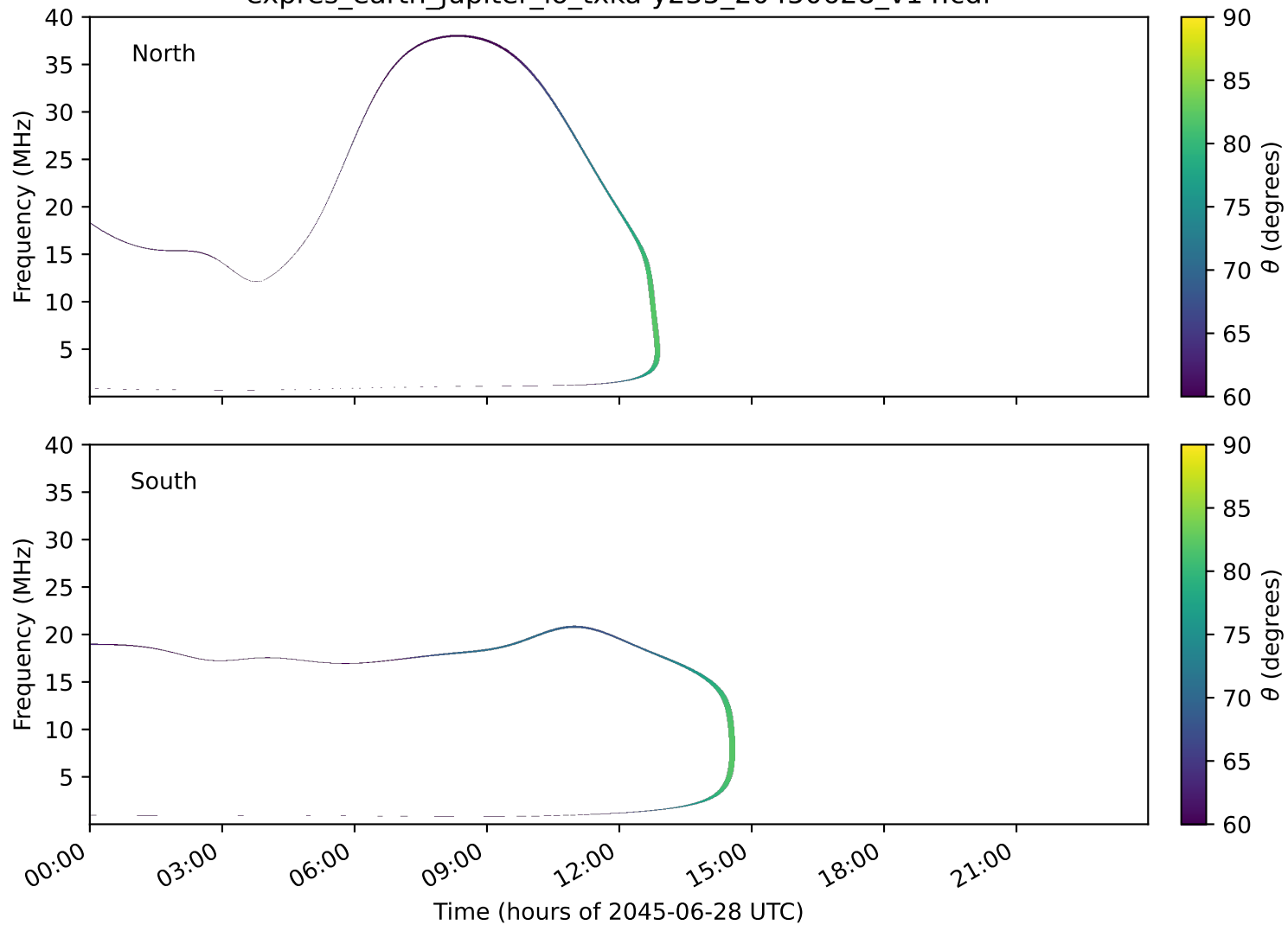
expres_earth_jupiter_io_txka-y235_20450628_v14.cdf
