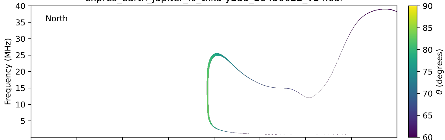
expres_earth_jupiter_io_txka-y235_20450622_v14.cdf
