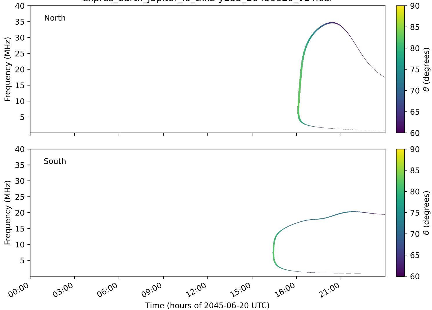
expres_earth_jupiter_io_txka-y235_20450620_v14.cdf
