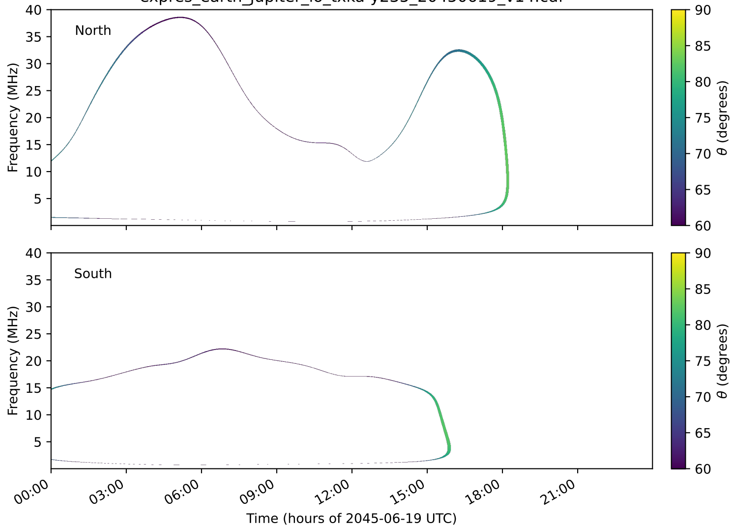
expres_earth_jupiter_io_txka-y235_20450619_v14.cdf
