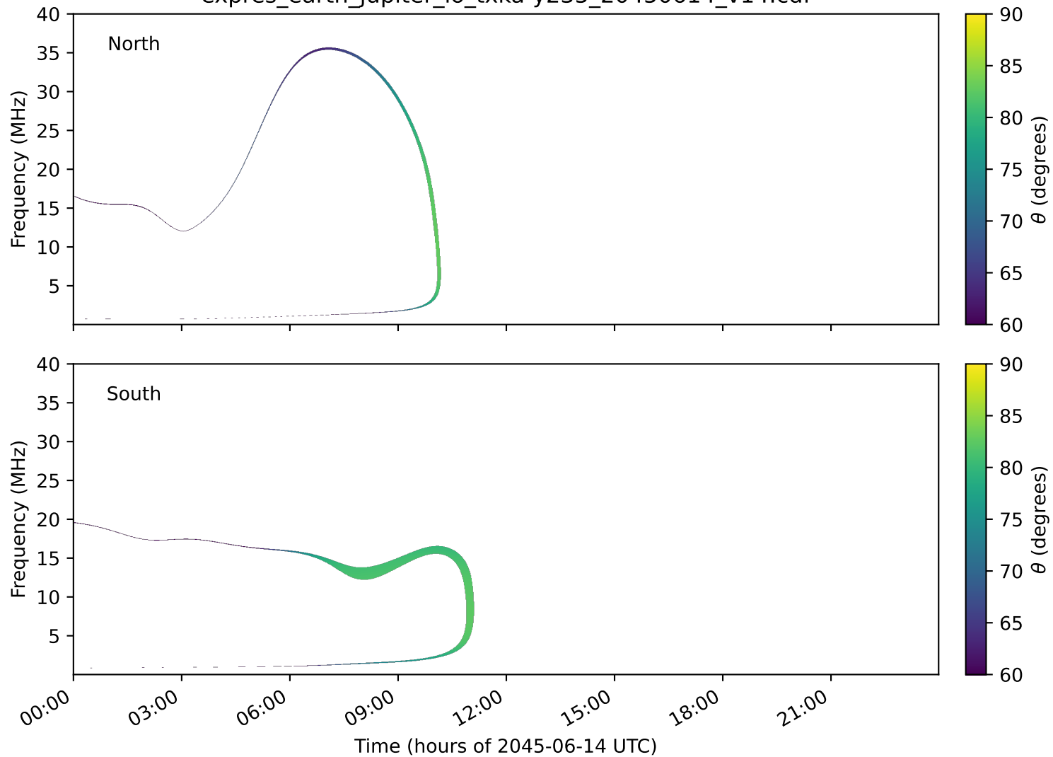
expres_earth_jupiter_io_txka-y235_20450614_v14.cdf
