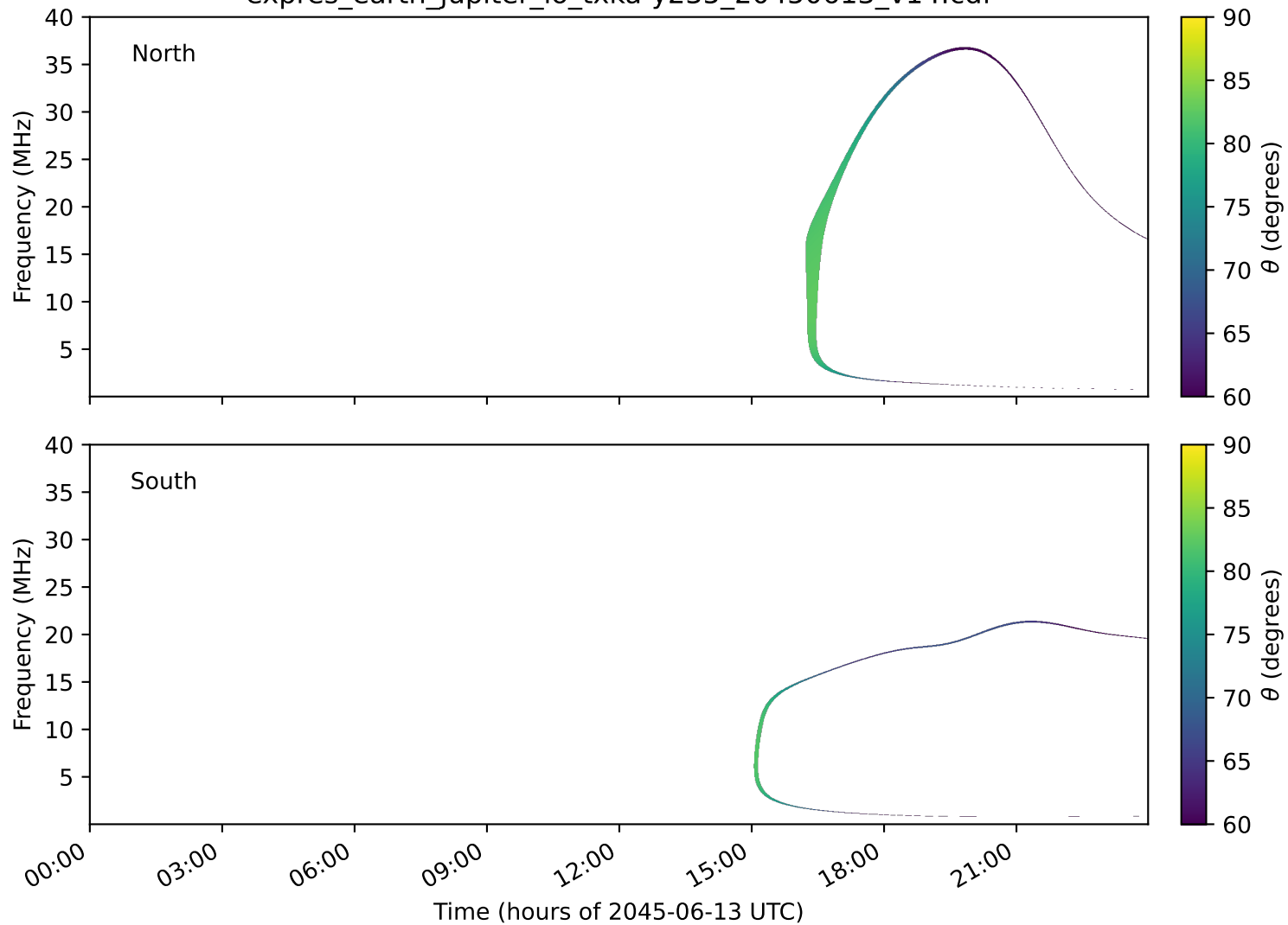
expres_earth_jupiter_io_txka-y235_20450613_v14.cdf
