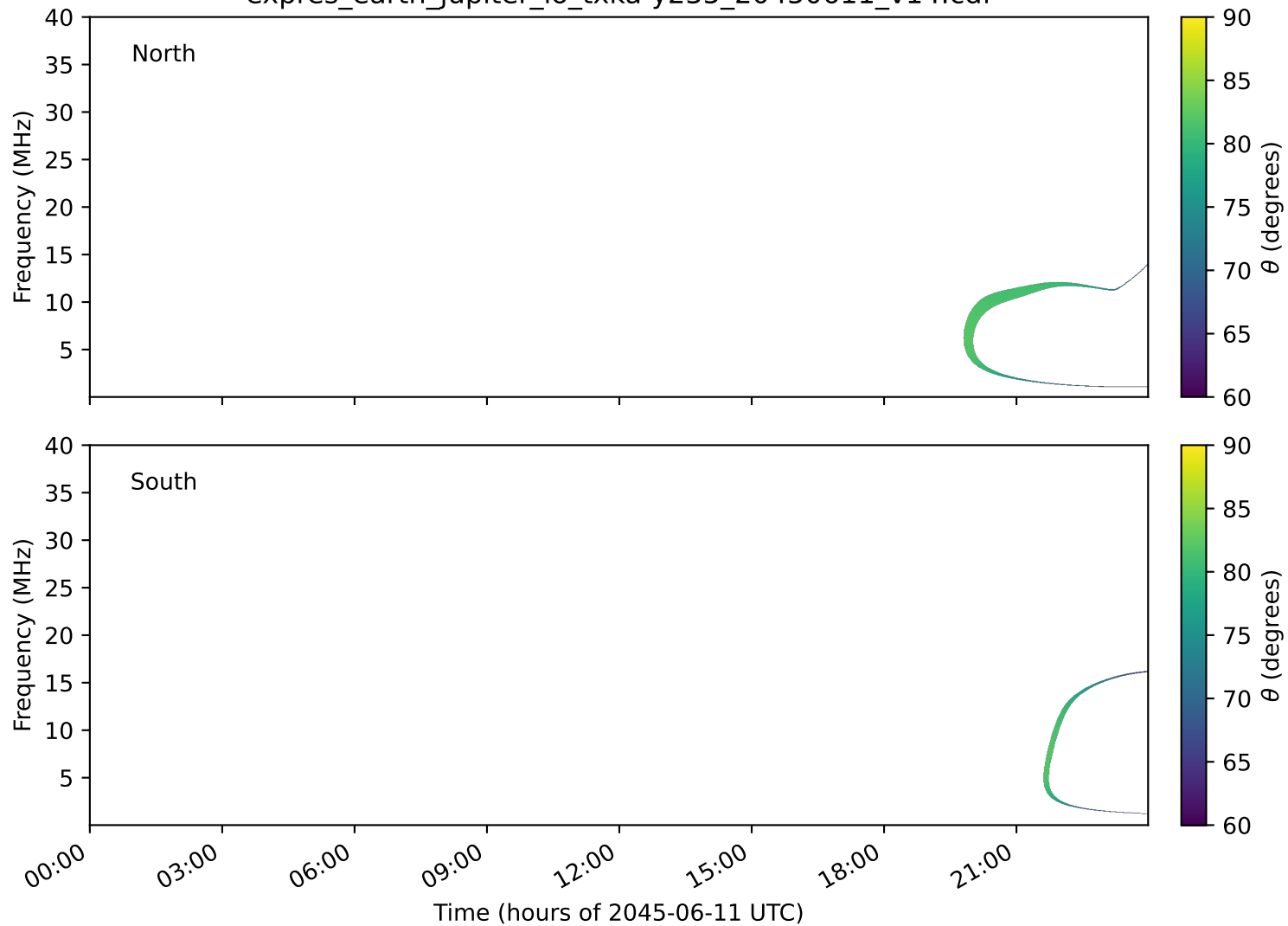
expres_earth_jupiter_io_txka-y235_20450611_v14.cdf
