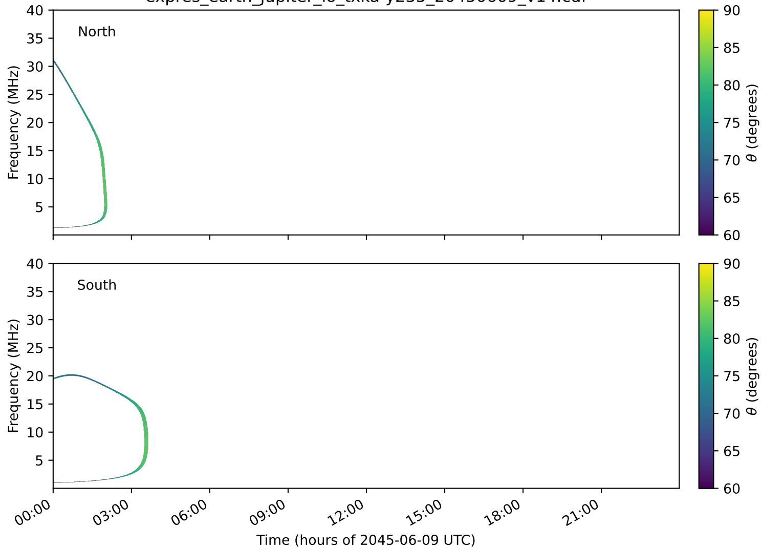
expres_earth_jupiter_io_txka-y235_20450609_v14.cdf
