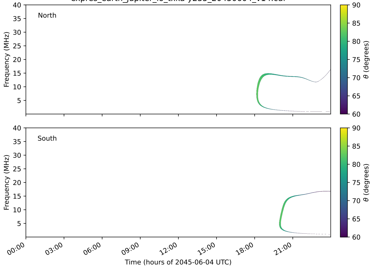
expres_earth_jupiter_io_txka-y235_20450604_v14.cdf
