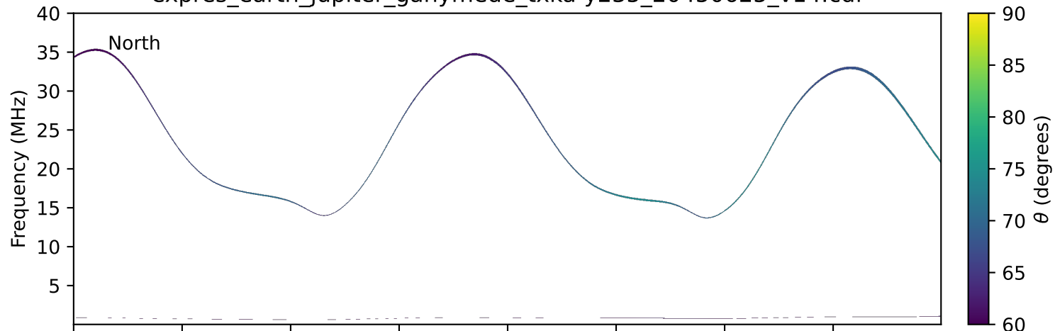
expres_earth_jupiter_ganymede_txka-y235_20450625_v14.cdf
