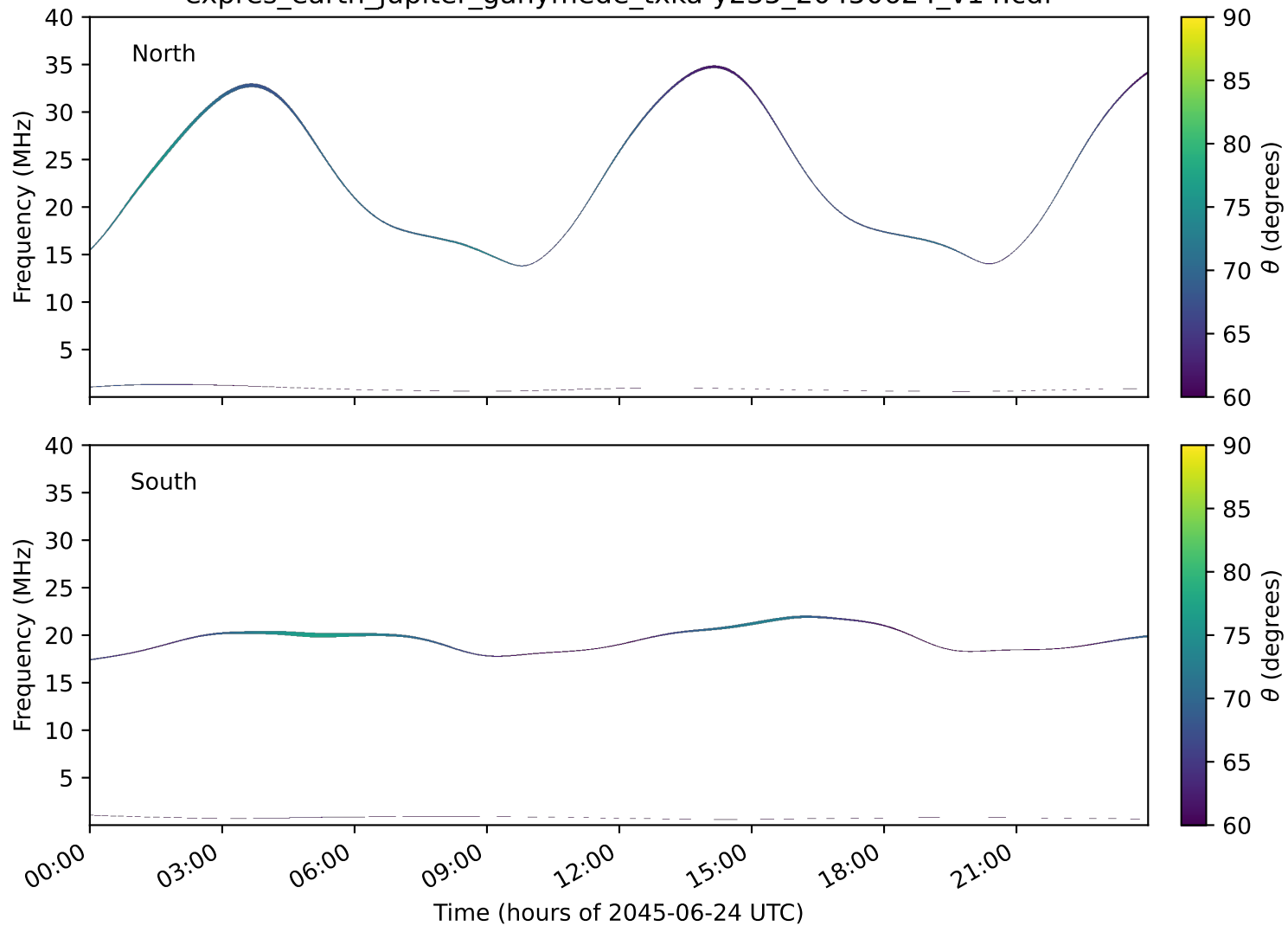
expres_earth_jupiter_ganymede_txka-y235_20450624_v14.cdf
