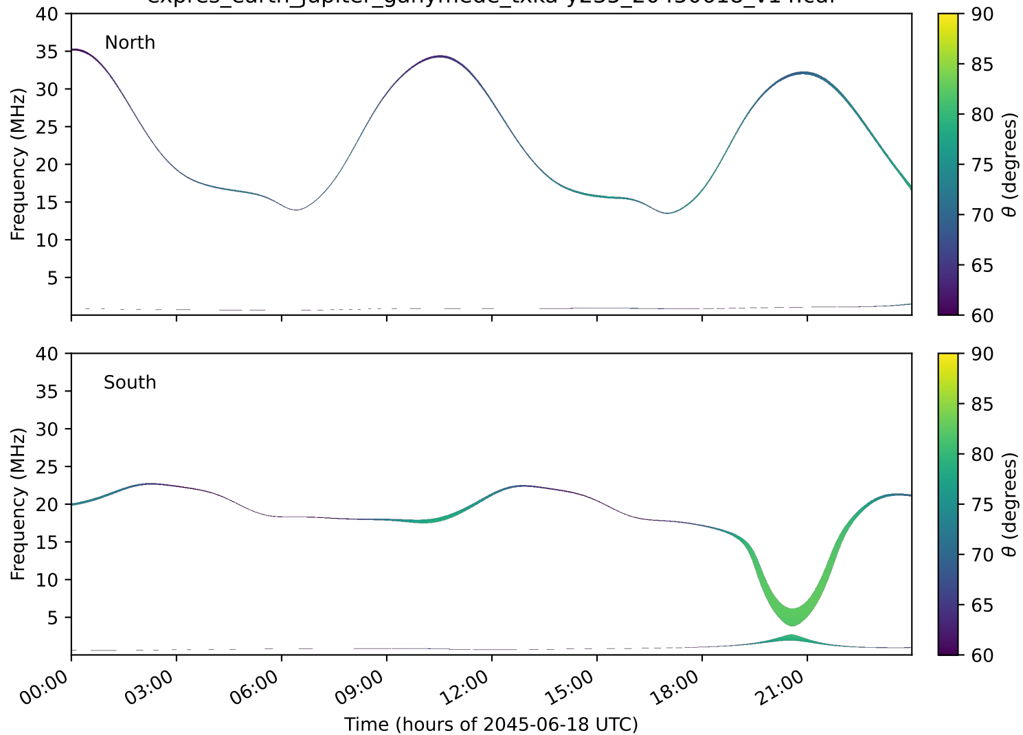
expres_earth_jupiter_ganymede_txka-y235_20450618_v14.cdf
