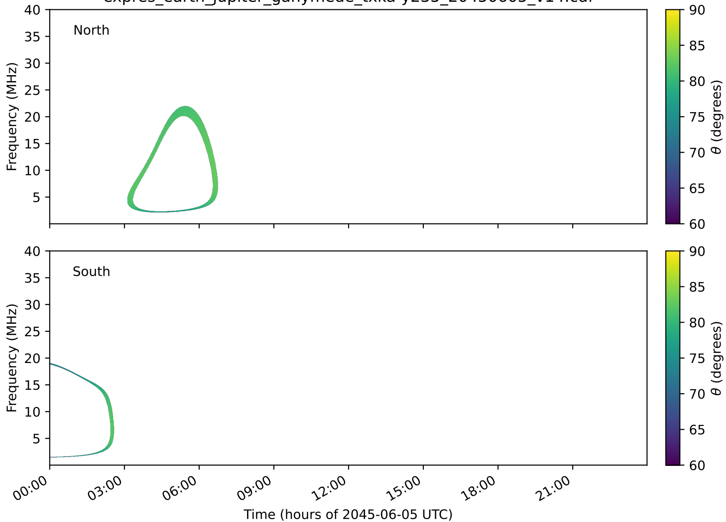
expres_earth_jupiter_ganymede_txka-y235_20450605_v14.cdf
