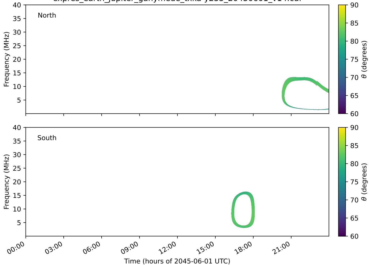
expres_earth_jupiter_ganymede_txka-y235_20450601_v14.cdf
