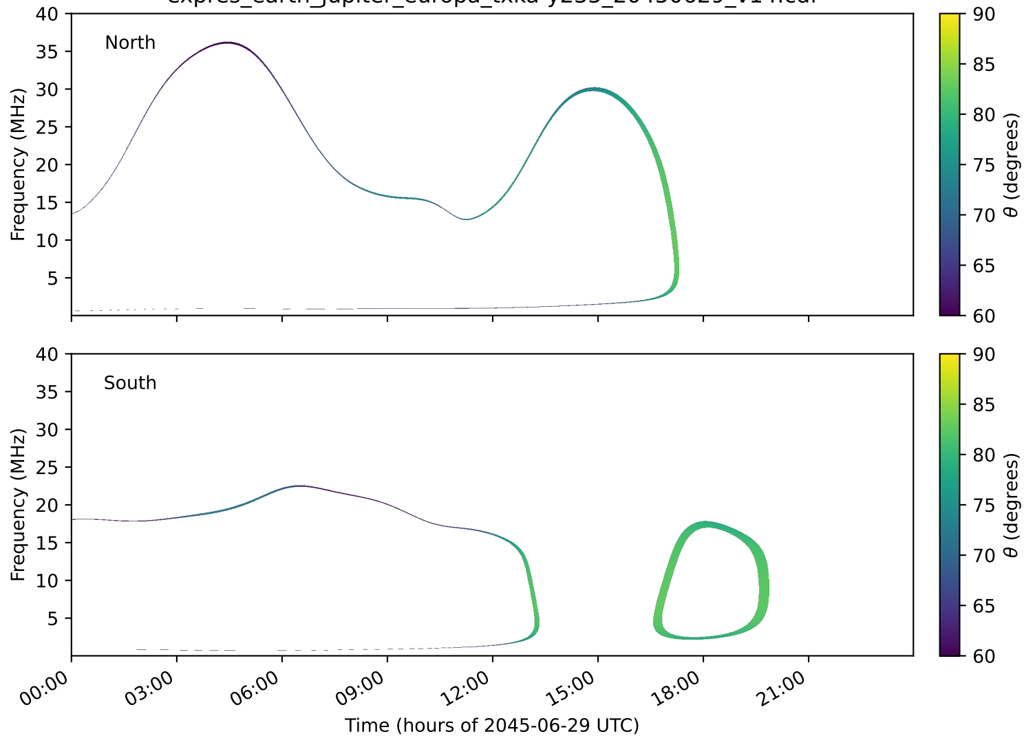
expres_earth_jupiter_europa_txka-y235_20450629_v14.cdf
