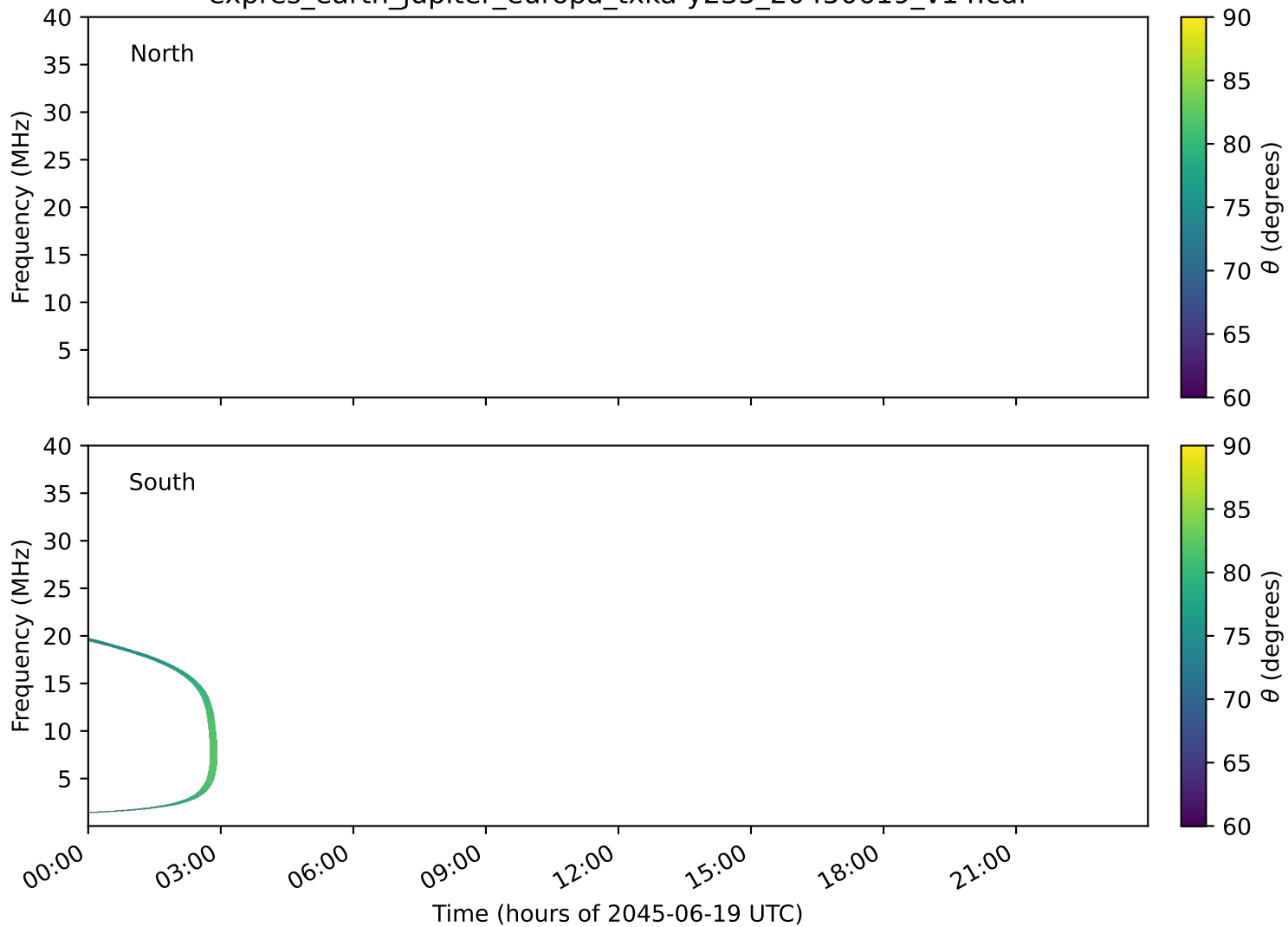
expres_earth_jupiter_europa_txka-y235_20450619_v14.cdf
