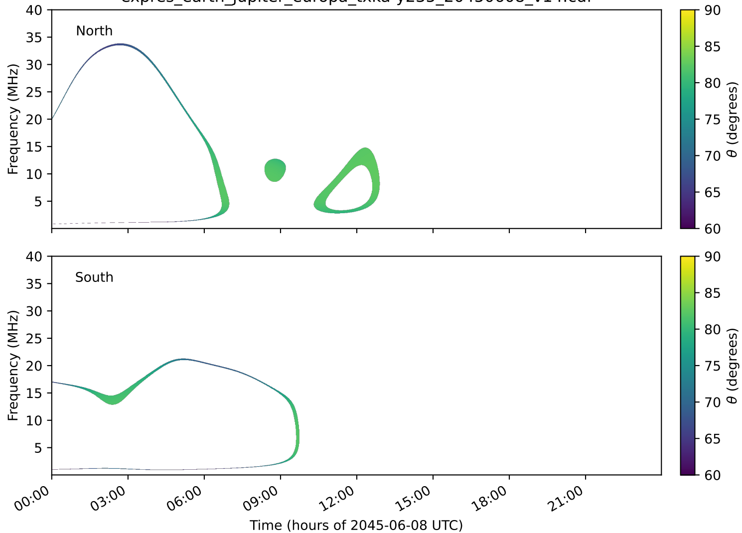
expres_earth_jupiter_europa_txka-y235_20450608_v14.cdf
