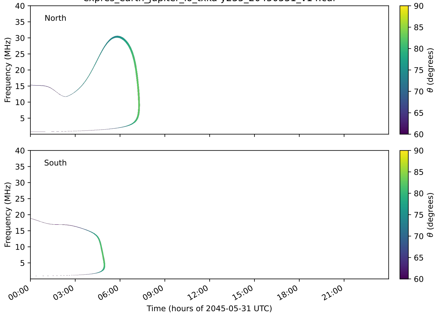
expres_earth_jupiter_io_txka-y235_20450531_v14.cdf
