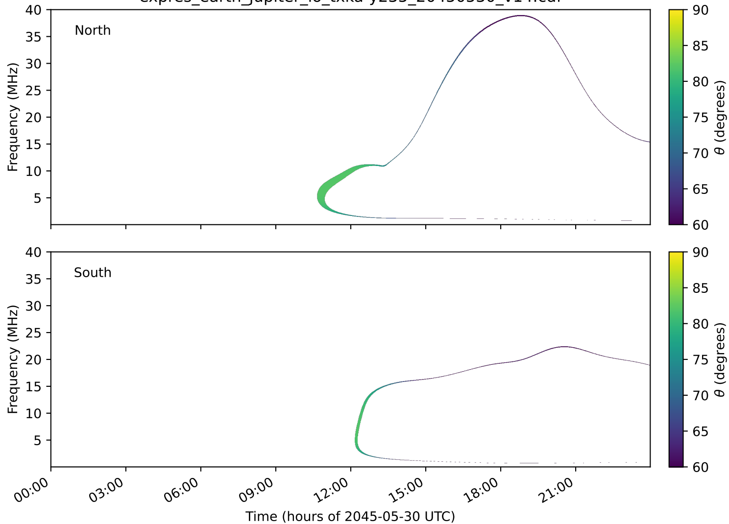
expres_earth_jupiter_io_txka-y235_20450530_v14.cdf
