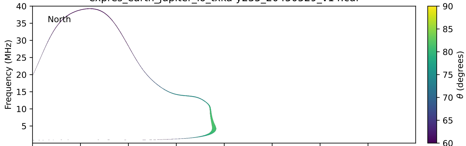
expres_earth_jupiter_io_txka-y235_20450529_v14.cdf
