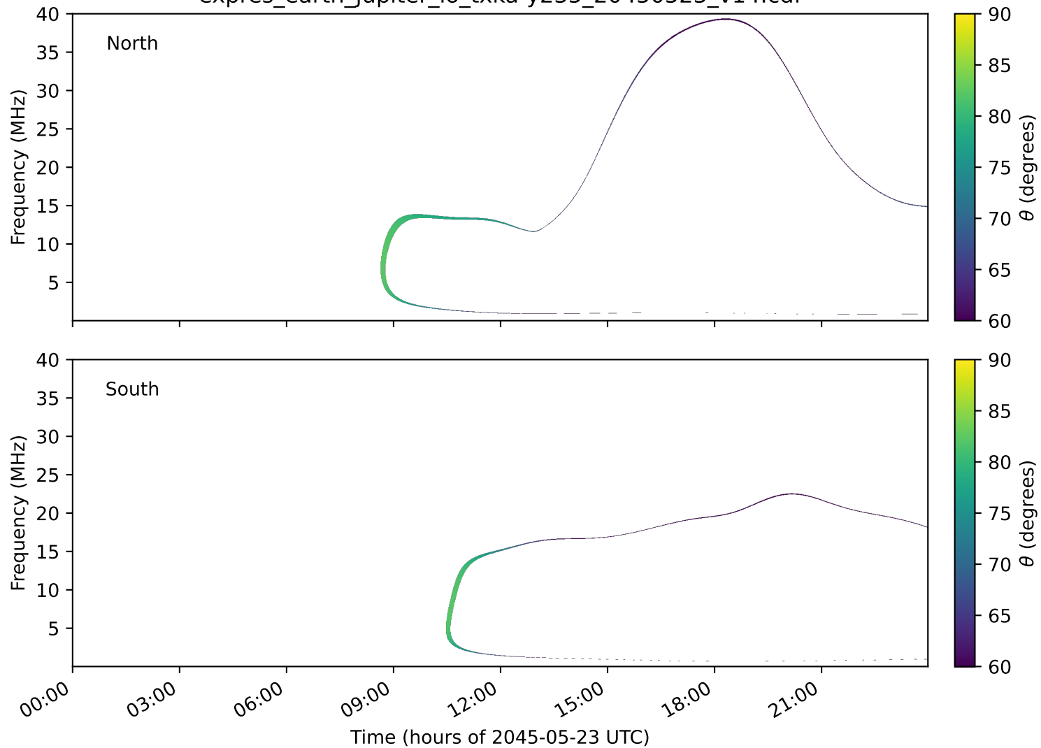
expres_earth_jupiter_io_txka-y235_20450523_v14.cdf
