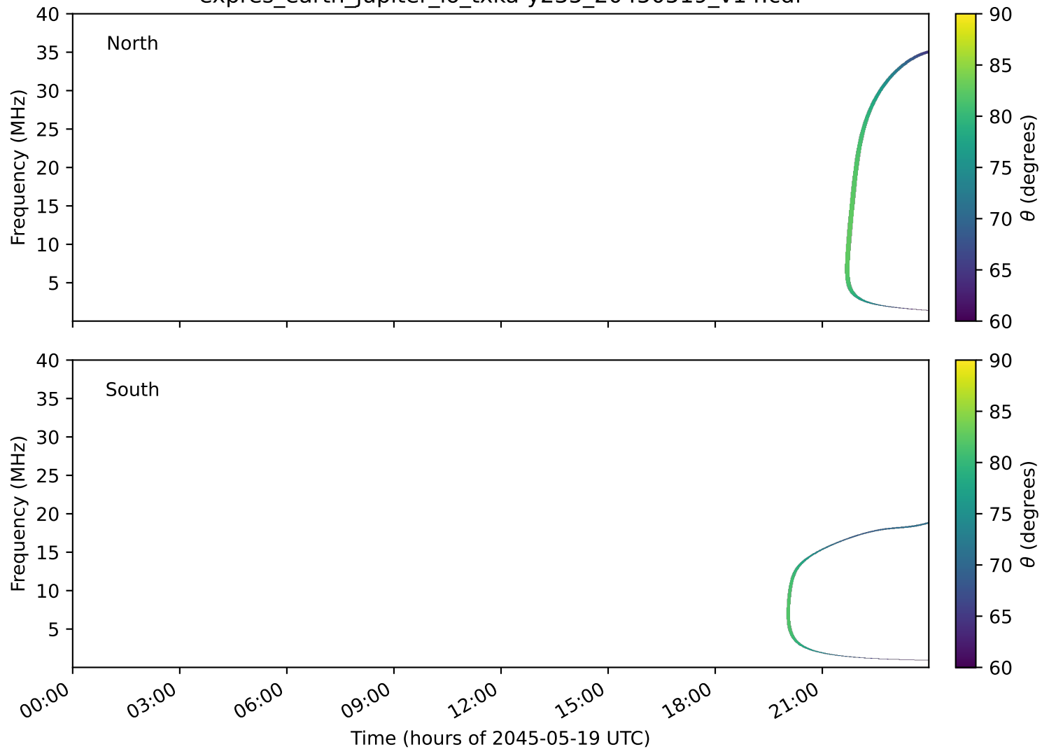
expres_earth_jupiter_io_txka-y235_20450519_v14.cdf
