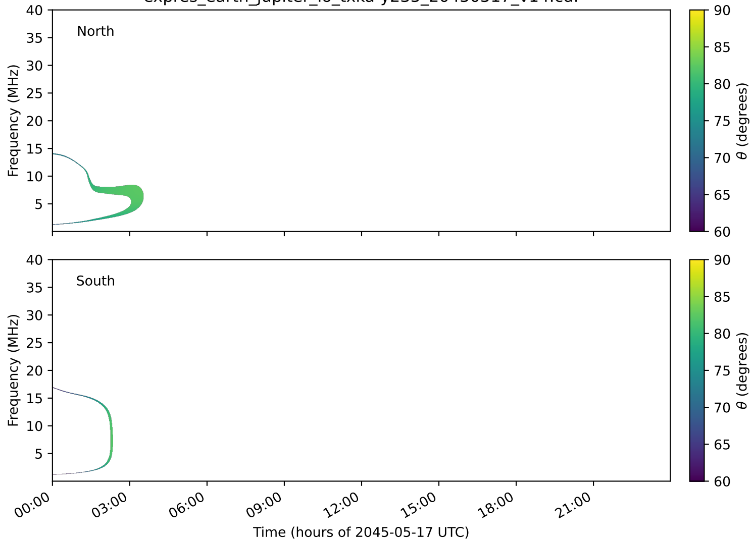
expres_earth_jupiter_io_txka-y235_20450517_v14.cdf
