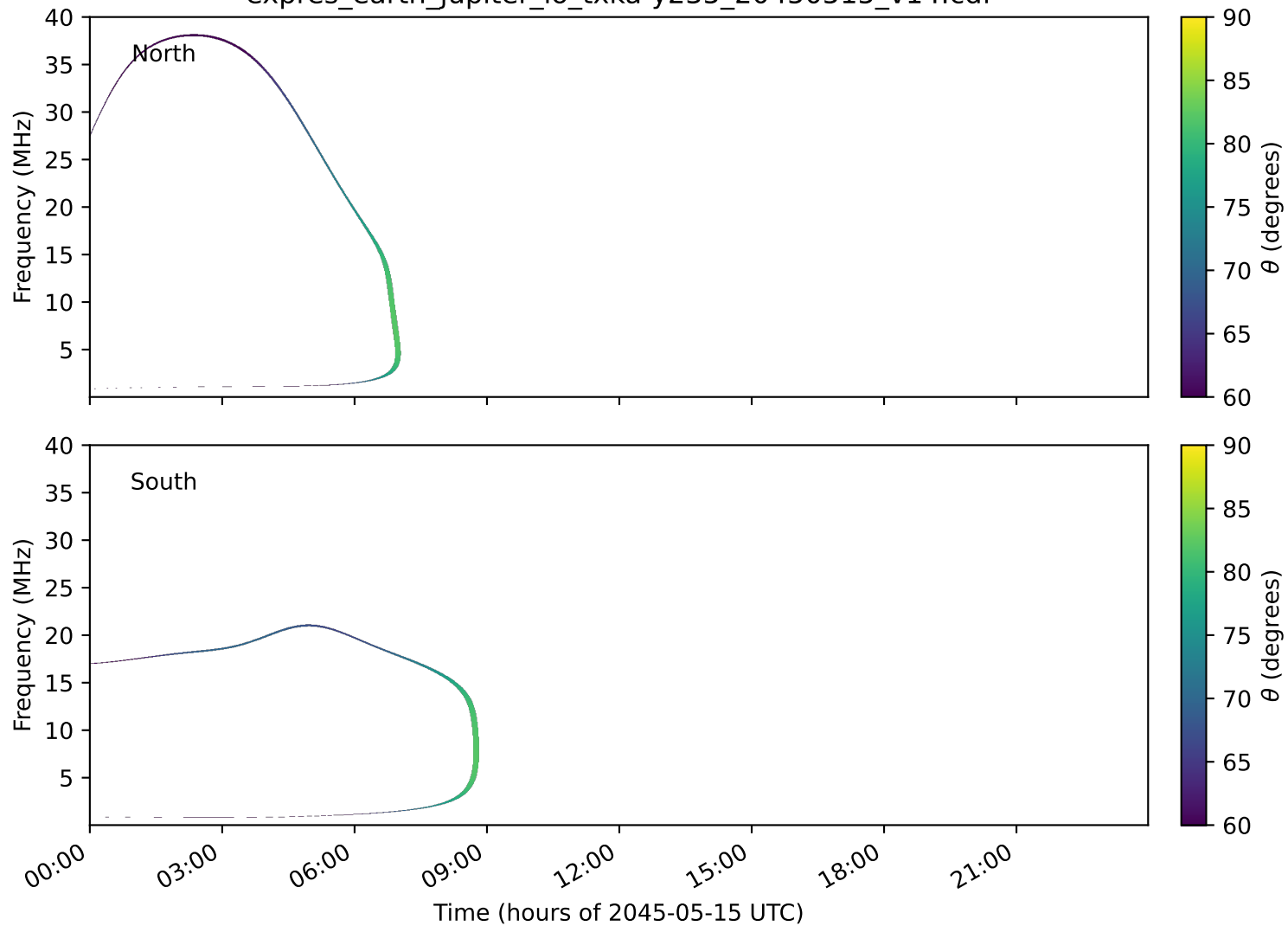
expres_earth_jupiter_io_txka-y235_20450515_v14.cdf
