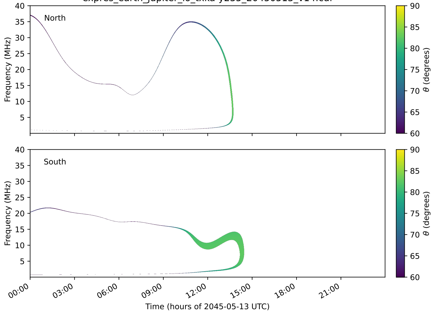
expres_earth_jupiter_io_txka-y235_20450513_v14.cdf
