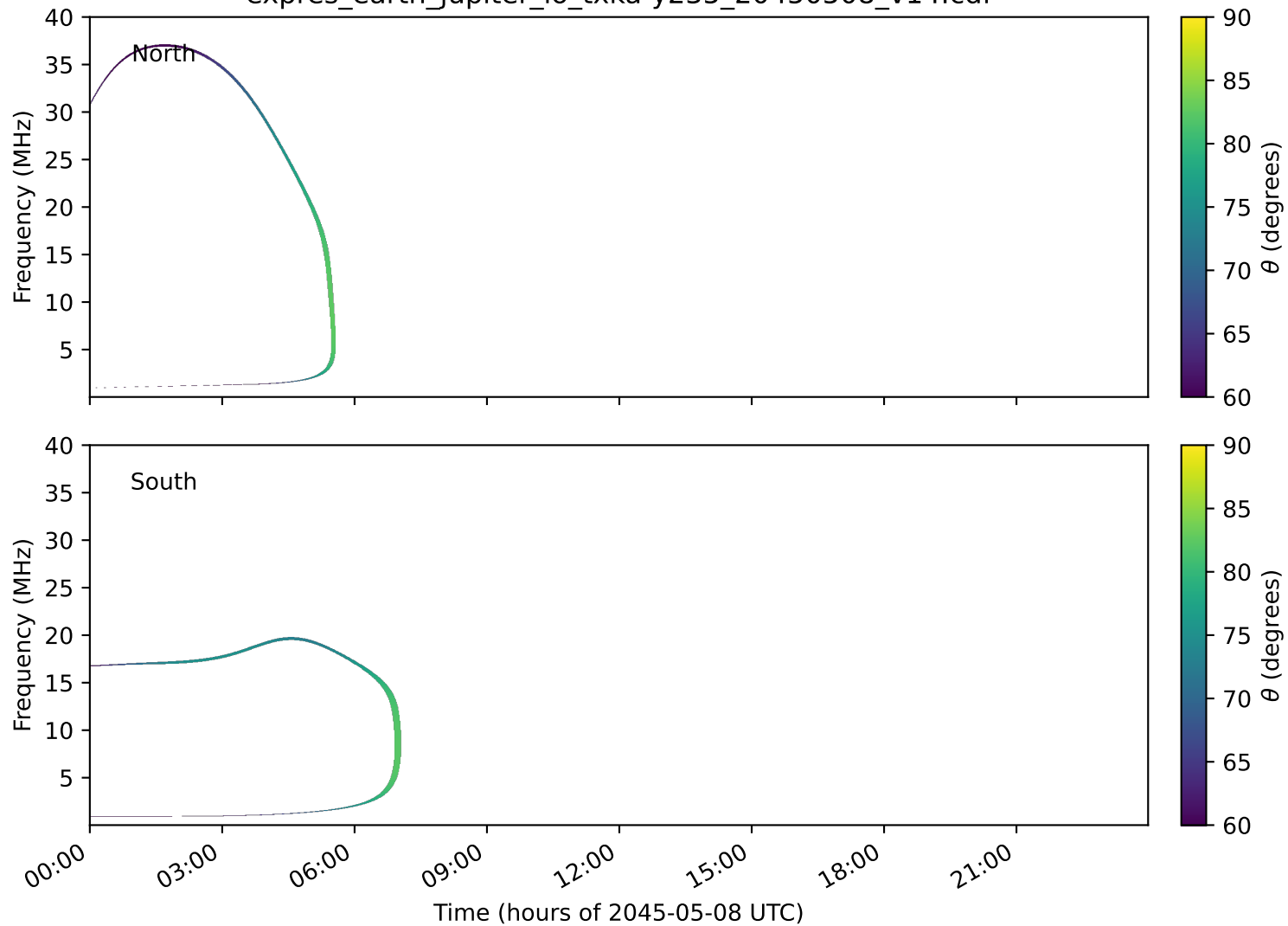
expres_earth_jupiter_io_txka-y235_20450508_v14.cdf
