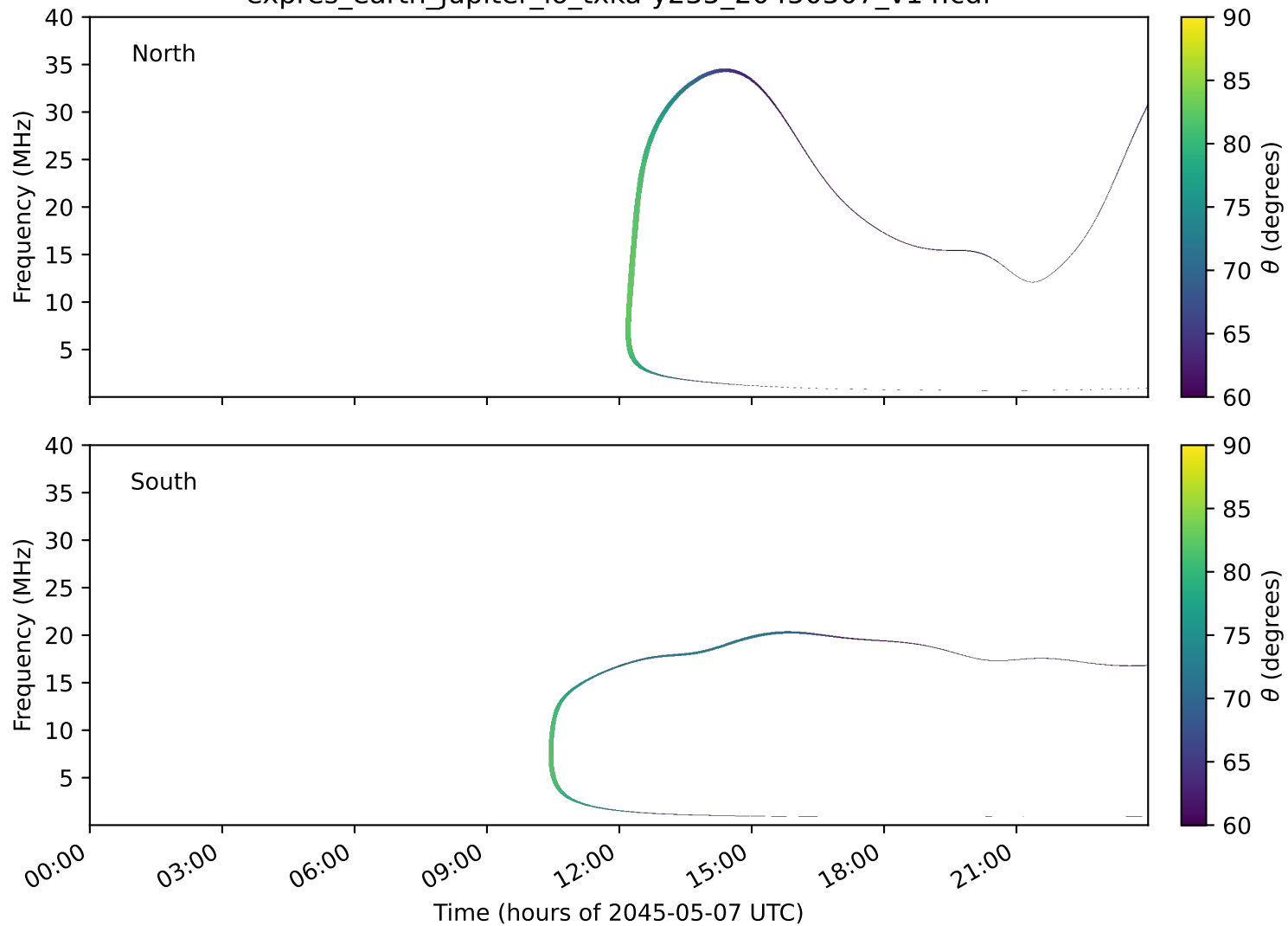
expres_earth_jupiter_io_txka-y235_20450507_v14.cdf
