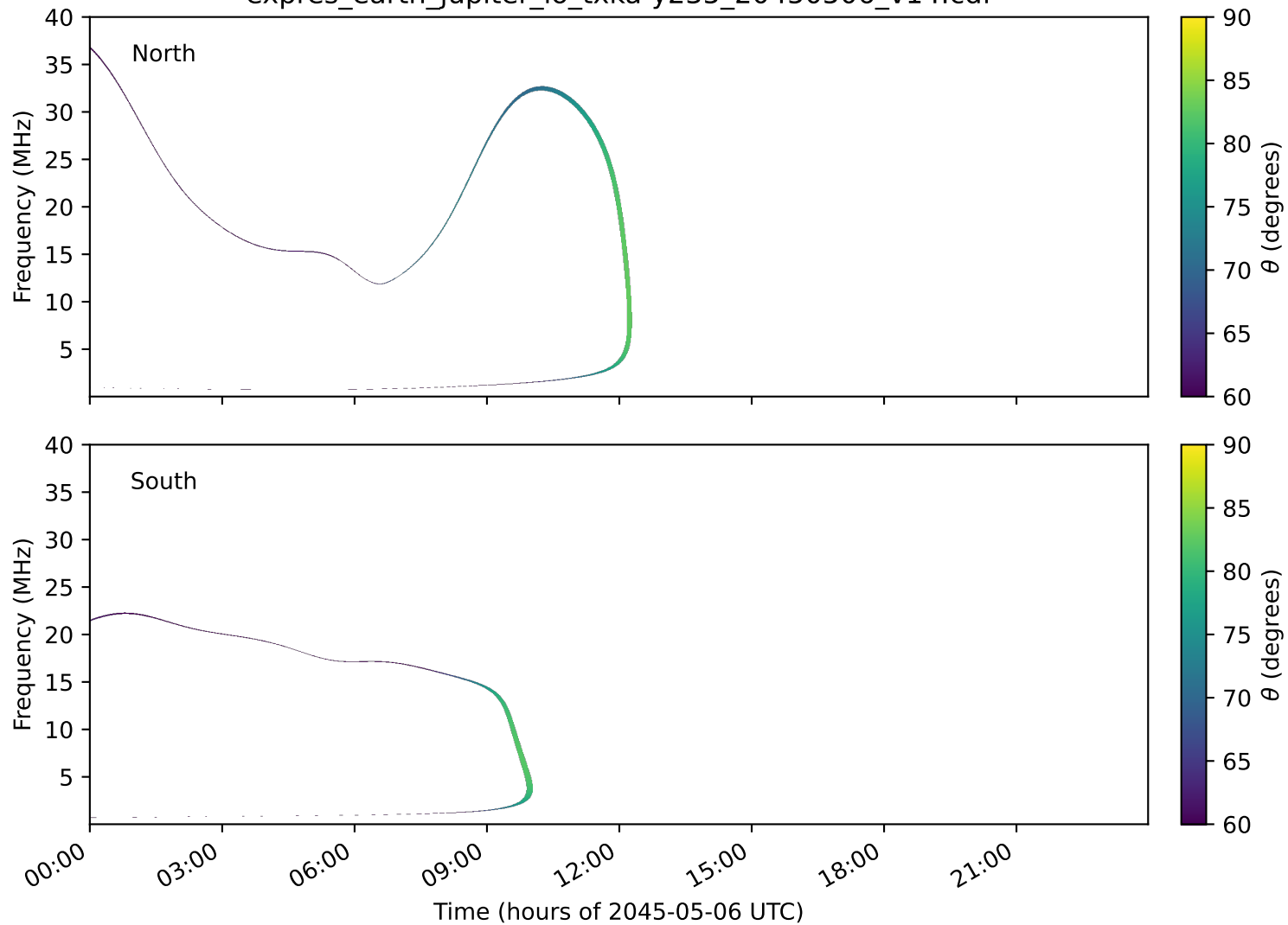
expres_earth_jupiter_io_txka-y235_20450506_v14.cdf
