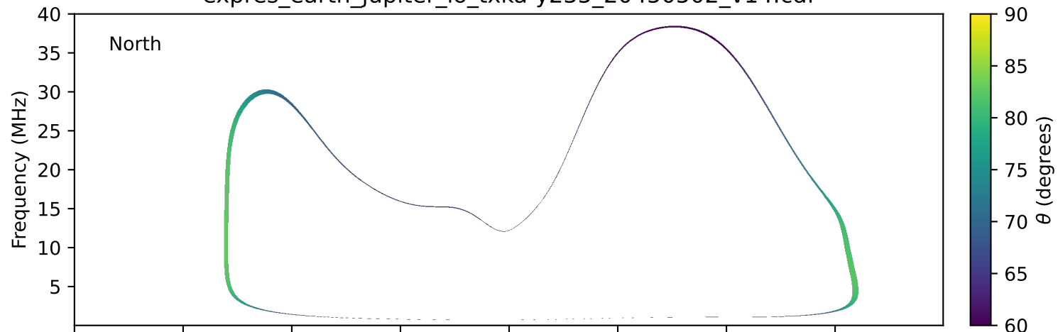
expres_earth_jupiter_io_txka-y235_20450502_v14.cdf
