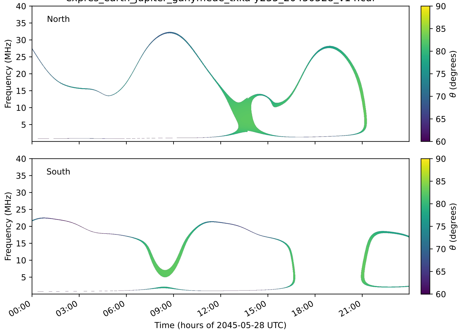
expres_earth_jupiter_ganymede_txka-y235_20450528_v14.cdf
