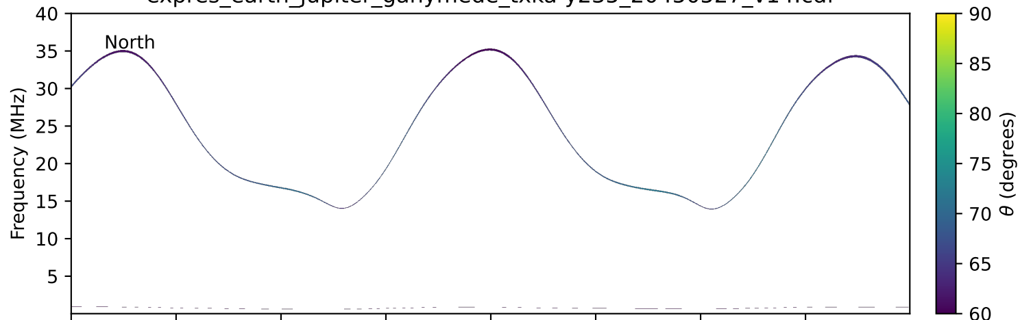
expres_earth_jupiter_ganymede_txka-y235_20450527_v14.cdf
