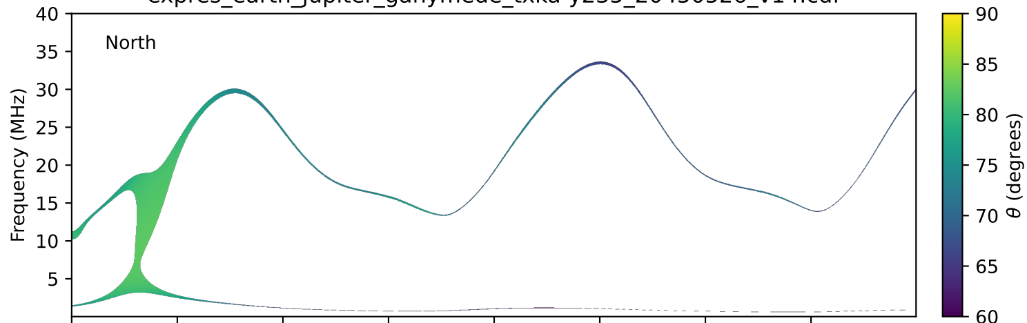
expres_earth_jupiter_ganymede_txka-y235_20450526_v14.cdf
