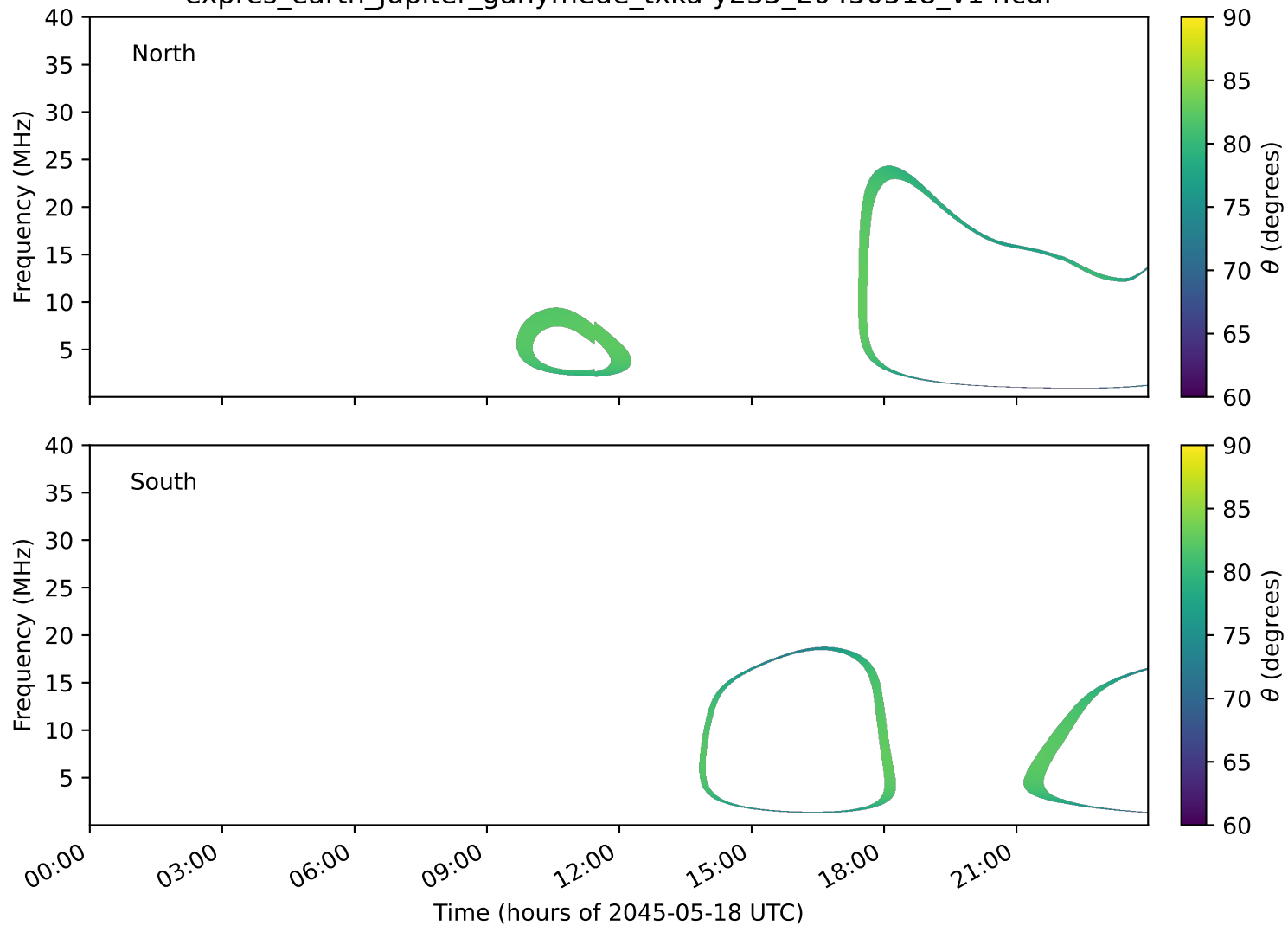
expres_earth_jupiter_ganymede_txka-y235_20450518_v14.cdf
