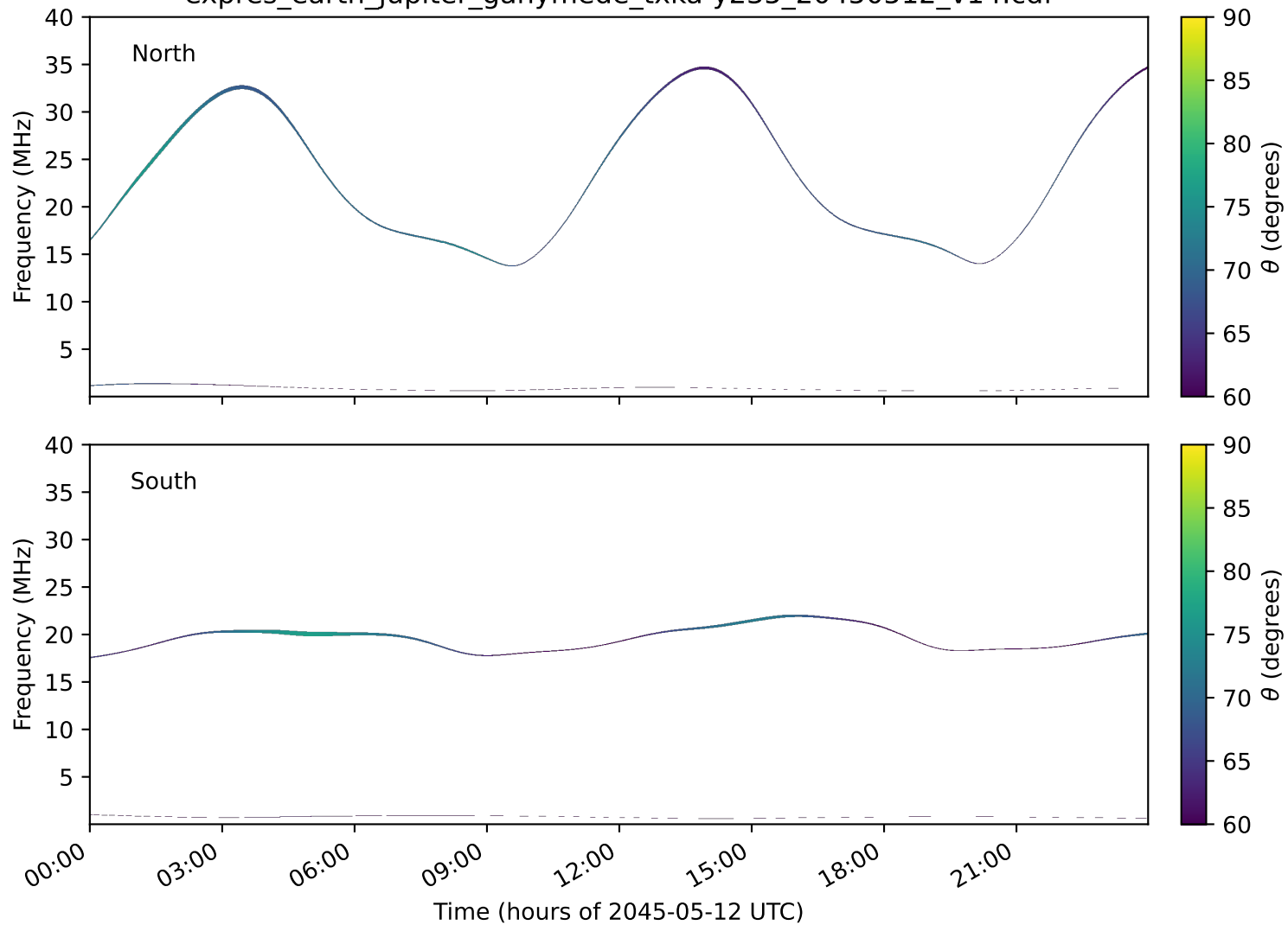
expres_earth_jupiter_ganymede_txka-y235_20450512_v14.cdf
