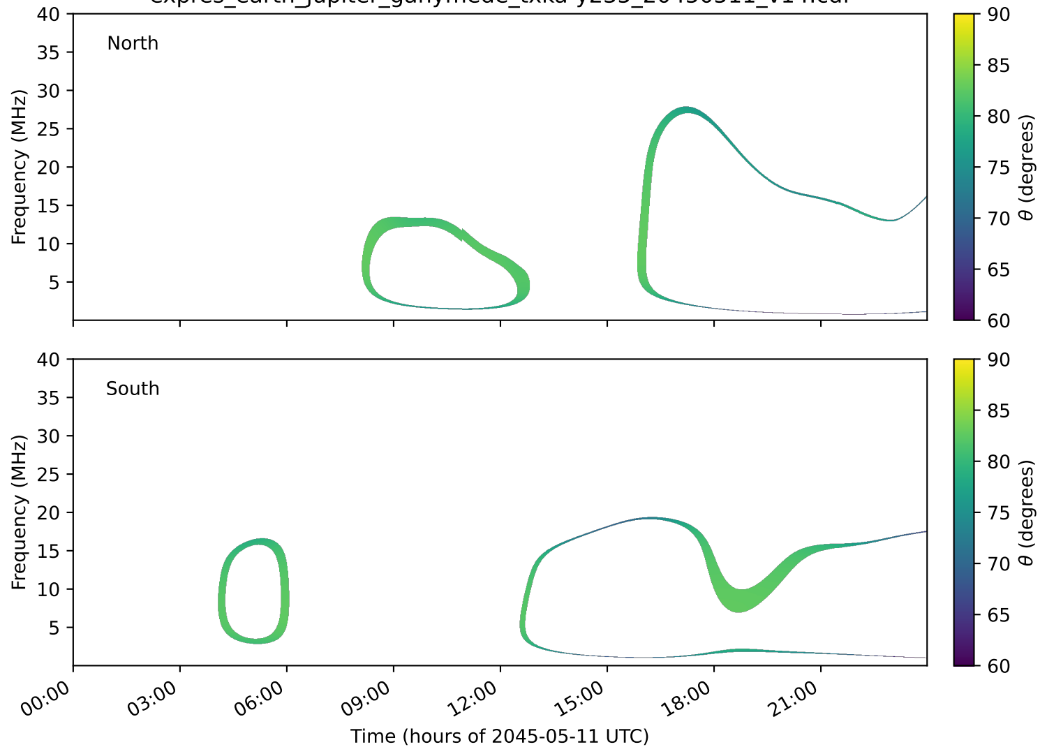
expres_earth_jupiter_ganymede_txka-y235_20450511_v14.cdf
