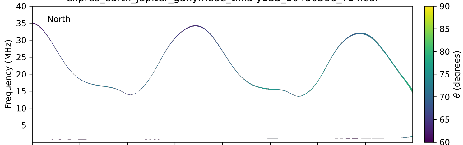
expres_earth_jupiter_ganymede_txka-y235_20450506_v14.cdf
