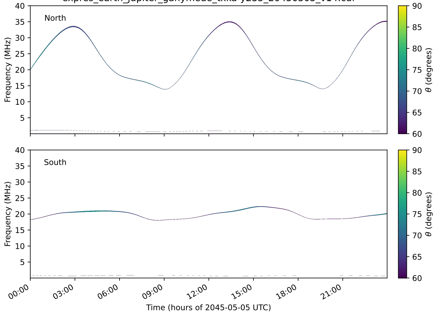
expres_earth_jupiter_ganymede_txka-y235_20450505_v14.cdf
